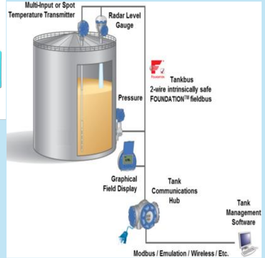
Complete Tank Gauging Solution for Oil Tank Farms (In Progress)
