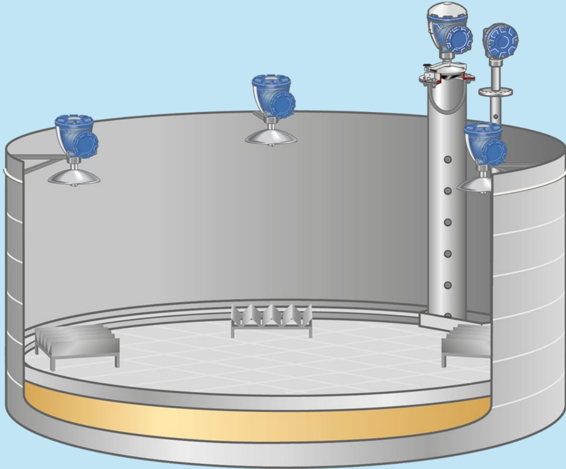
Complete Tank Gauging Solution, E&I Supply and Installation Oil Tank Farm in Sharjah, UAE
